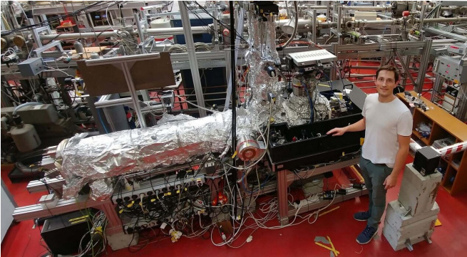
A photo of the COLTRIMS reaction microscope built by Alexander Hartung as part of his doctoral research in the experiment hall of the Faculty of Physics. Credit: Alexander Hartung
