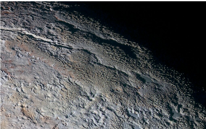
Blade-like features called penitentes, here observed on the surface of Pluto, would provide the required reflective efficiency for the radar brightness seen at Mimas, Tethys and Enceladus. However, it's not clear that there is enough solar energy to sublimate the ice and form such structures. Credit: NASA/JHUAPL/SwRI
