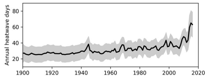
Yearly count of marine heatwave days from 1900 to 2016, as a global average. Credit: Eric Oliver
