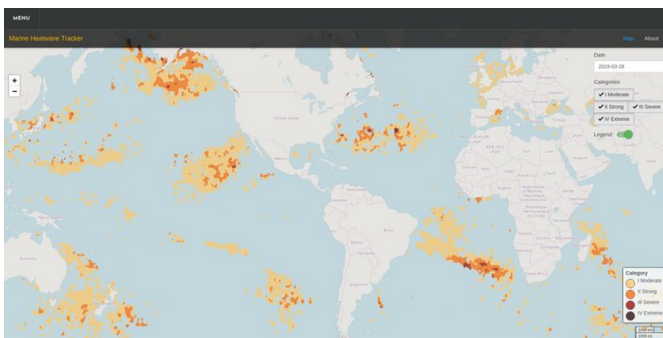
Screenshot from live marine heatwave tracker ( marineheatwaves.org/tracker ) showing the global distribution of marine heatwaves on Mar. 28, 2019. Credit: Eric Oliver
