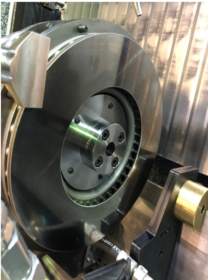
A finished brake disc coated with the EHLA process. Credit: Buderus Schleiftechnik, Aßlar, Germany | HPL Technologies, Aachen, Germany
