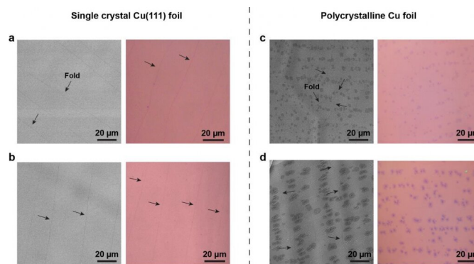
(a-b) (left panel) SEM images of adlayer-free single crystal graphene films on Cu(111) foils and (right panel) optical images of the films after transfer to 300 nm SiO 2 /Si wafers. (c-d) (left panel) SEM images of polycrystalline graphene films with adlayers on polycrystalline Cu foils and (right panel) optical images of the films after transfer to 300 nm SiO 2 /Si wafers. CVD parameters for gas flow and pressure were as follows: (a, c) H 2 /CH 4 (200 sccm / 1 sccm) at 2.0 Torr; (b, d) H 2 /CH 4 (30 sccm / 30 sccm 0.1% CH 4 in Ar) at 30.0 Torr. The black arrows point to folds. Credit: Ulsan National Institute of Science and Technology (UNIST)
