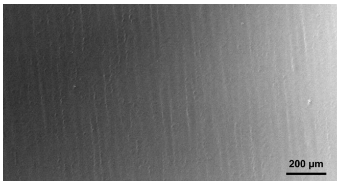
A large scale (~2.5 mm x 1.6 mm) SEM image of an adlayer-free single crystal graphene film on a Cu(111) foil. Credit: Ulsan National Institute of Science and Technology (UNIST)
