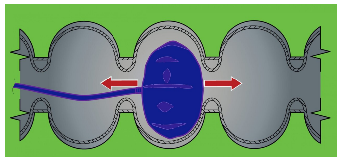
To stretch one cell of an accelerator cavity, a balloon is placed inside it and inflated. Credit: Diana Brandonisio
