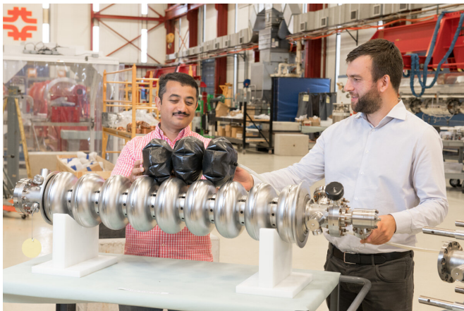
Fermilab engineers Mohamed Hassan, left, and Donato Passarelli stand near an accelerator cavity and the patented balloons used to tune, or reshape, the cavity from the inside. Credit: Reidar Hahn
