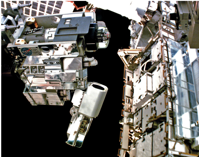
Robotic Refueling Mission 3's Multi-Function Tool 2, operated by Dextre, demonstrates robotic refueling operations on the outside of space station. Credit: NASA
