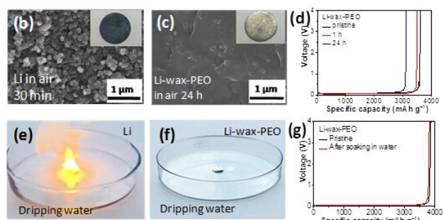
Diagram of the Li-wax-PEO and its stability in the air and water. Credit: Science China Press
