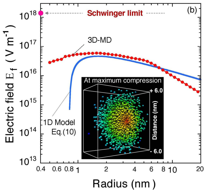
Fig.2 Comparison of the electrostatic fields between the 3D simulation and the model. The inset shows the proton distribution around the center (color-coded in accordance with the distance from the center). Credit: M. Murakami
