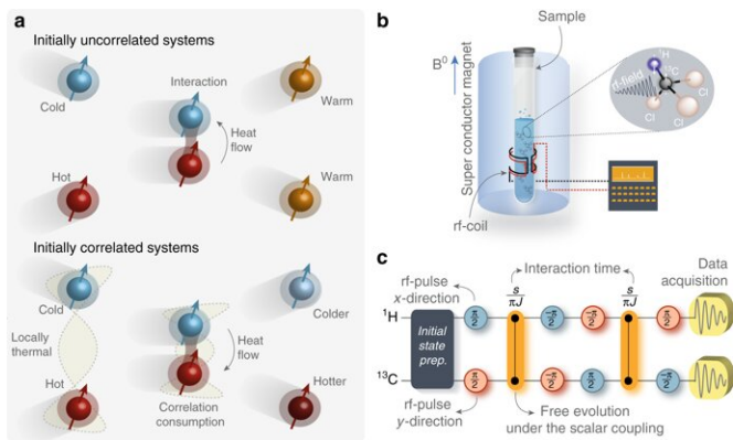
Fig. 1: Schematic of the experimental setup. a Heat flows from the hot to the cold spin (at thermal contact) when both are initially uncorrelated. This corresponds to standard thermodynamic. For initially quantum-correlated spins, heat is spontaneously transferred from the cold to the hot spin. The direction of heat flow is here reversed. b View of the magnetometer used in our NMR experiment. A superconducting magnet, producing a high-intensity magnetic field ( B^0 ) in the longitudinal direction, is immersed in a thermally shielded vessel in liquid He, surrounded by liquid N in another vacuum separated chamber. The sample is placed at the center of the magnet within the radio-frequency coil of the probe head inside a 5-mm glass tube. c Experimental pulse sequence for the partial thermalization process. The blue (black) circle represents x (y) rotations by the indicated angle. The orange connections represents a free evolution under the scalar coupling, H_{\text{HJC}} = \hbar J \sigma_x^{\text{H}} \sigma_z^{\text{C}} , between the ^1\text{H} and ^{13}\text{C} nuclear spins during the time indicated above the symbol. We have performed 22 samplings of the interaction time \tau in the interval 0 to 2.32 ms. Credit: Nature Communications, from: Reversing the direction of heat flow using quantum correlations
