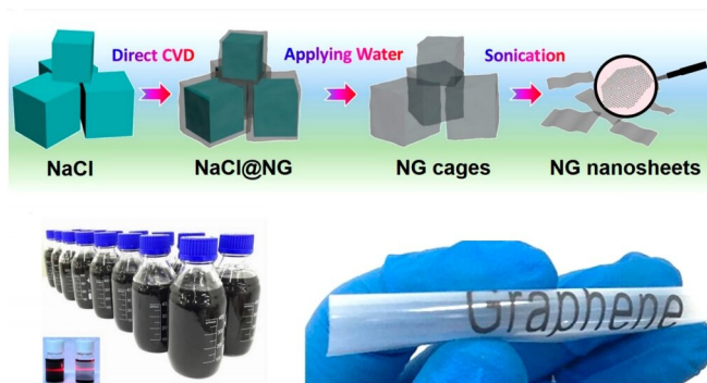
(Top) The salt-templated process of synthesizing graphene nanosheets into ink. (Bottom) The ink and printed demonstration. Credit: Wei et al. ©2019 American Chemical Society
