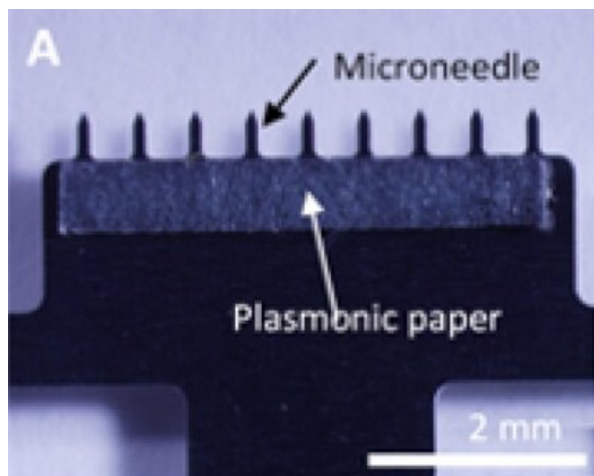
This microneedle patch can collect interstitial fluid onto plasmonic paper for analysis. Credit: Adapted from ACS Sensors 2019, DOI: 10.1021/acssensors.9b00258
