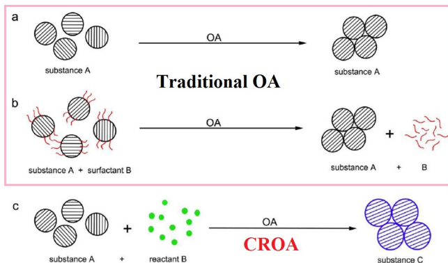
Fig. 1a, Traditional oriented attachment (OA) of nanoparticles to form a single crystal. Fig. 1b, With the aid of surfactants (red wavy lines) a single crystal can also form via traditional OA. Fig. 1c, The Chemical Reaction-directed OA (CROA) process. Credit: LIU Yongfei and YANG Yong
