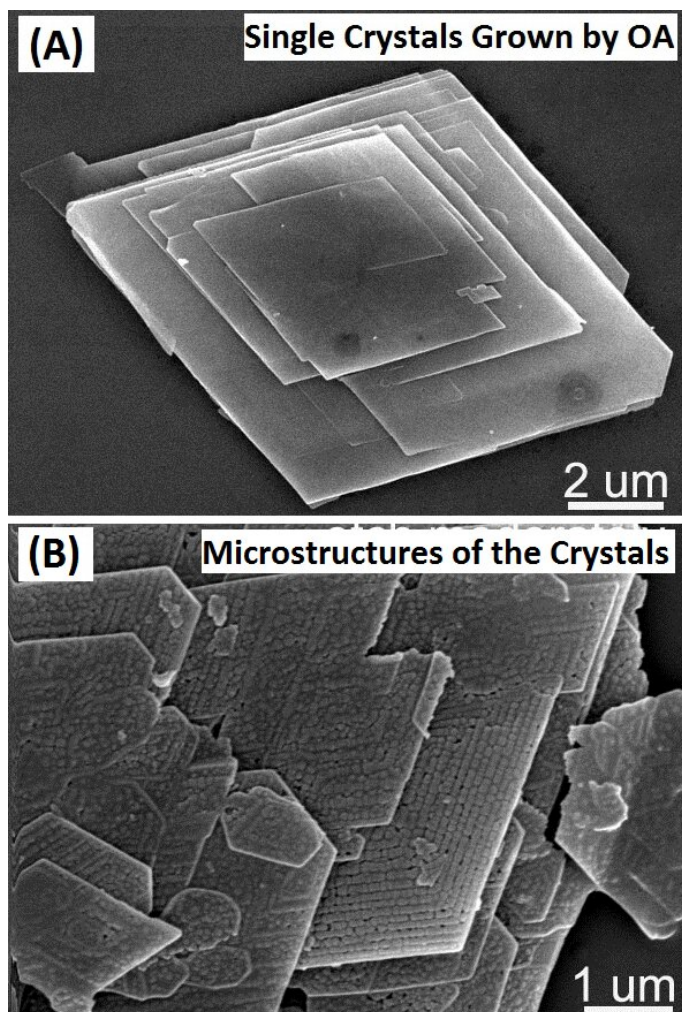
(A) Single crystals grown by OA; (B) Microstructures of the crystals, which show the oriented alignment of the nanoparticles. Credit: YANG Yong
