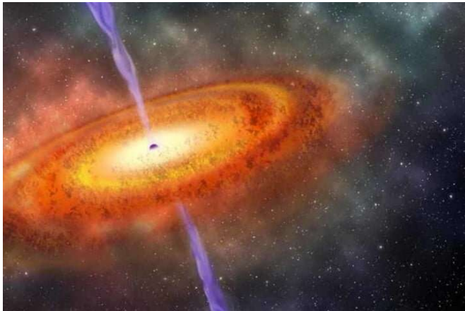
Quasar. Credit: Robin Dienel/Carnegie Institution for Science
