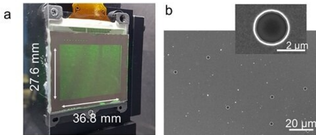
The actual 3D holographic display, and an electron microscope image of the non-periodic pinholes. Credit: KAIST
