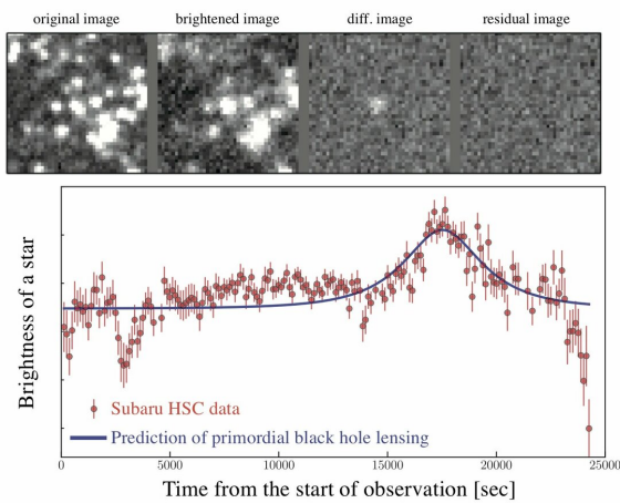
Figure 3: Data from the star which showed characteristics of being magnified by a potential gravitational lens, possibly by a primordial black hole. About 4 hours after data taking on the Subaru Telescope began, one star began to shine brighter. Less than an hour later, the star reached peak brightness before becoming dimmer. Credit: Niikura et al.
