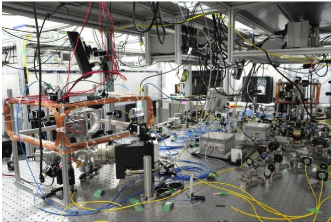
Experimental device for an all-fiber, coupled cavities-QED system. Credit: Aoki Laboratory, Waseda University
