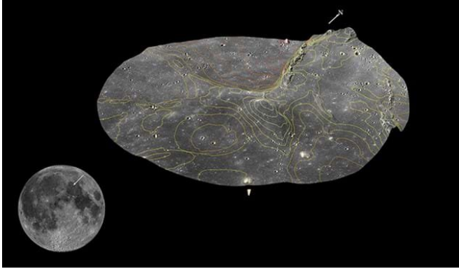
The topography of the 140 km (87 mi) diameter area containing the potential lunar landing sites in Mare Serenitatis (arrow). Darker colors indicate lower elevation. Credit: Weizmann Institute of Science
