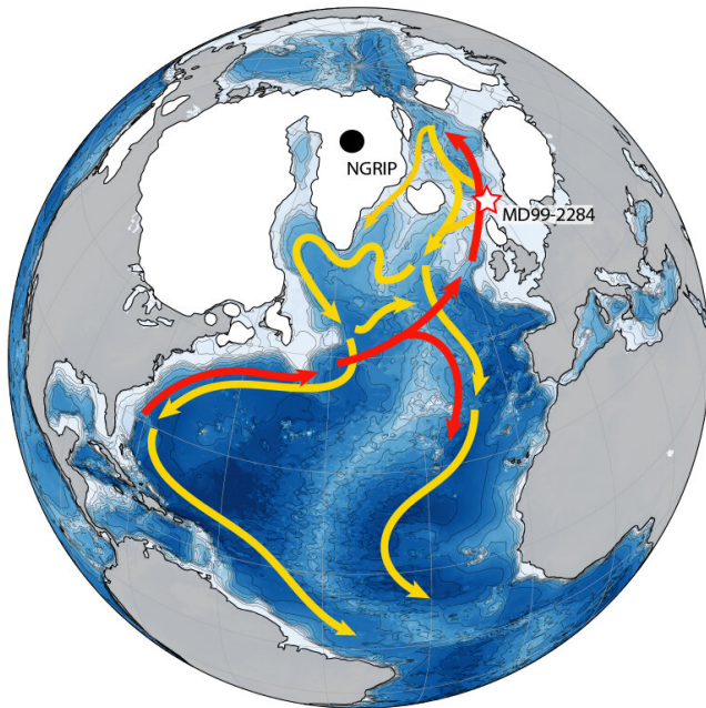
Simplified diagram of the Atlantic Meridional Overturning Circulation. It carries warm water from the tropics (red arrows) into the North Atlantic, where the water cools and sinks before flowing back south (yellow arrows). This pattern plays an important role in regulating climate in the North Atlantic as well as the rest of the world. Credit: Muschitiello et al. , Nature Communications , 2019
