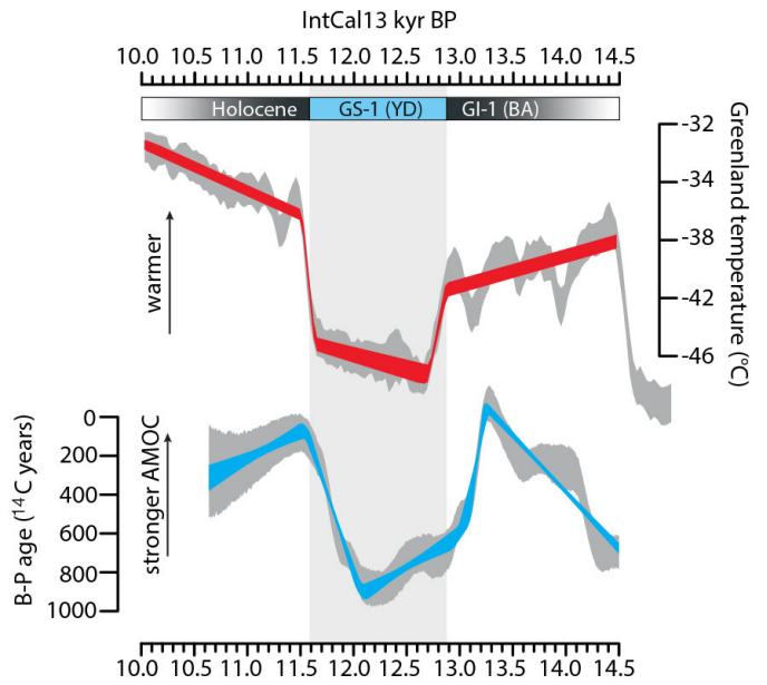
The study finds that changes in AMOC strength (blue line) began hundreds of years before the sharp and abrupt temperature changes over Greenland (red line) that mark the beginning and end of the hemispheric cold snap known as the Younger Dryas period (shown here as a gray column). Credit: Muschitiello et al.
