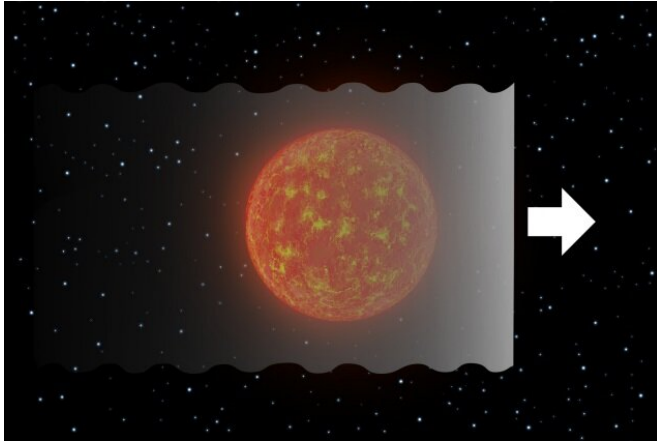
Artist's conception of the knife-edge dust sheet passing in front of EPIC 204376071. Credit: Danielle Futselaar; artsource.nl
