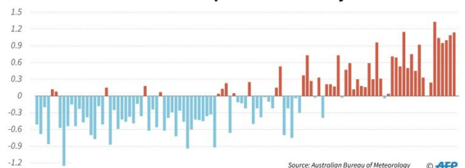
Australia: annual mean temperature anomaly 1910-2018
