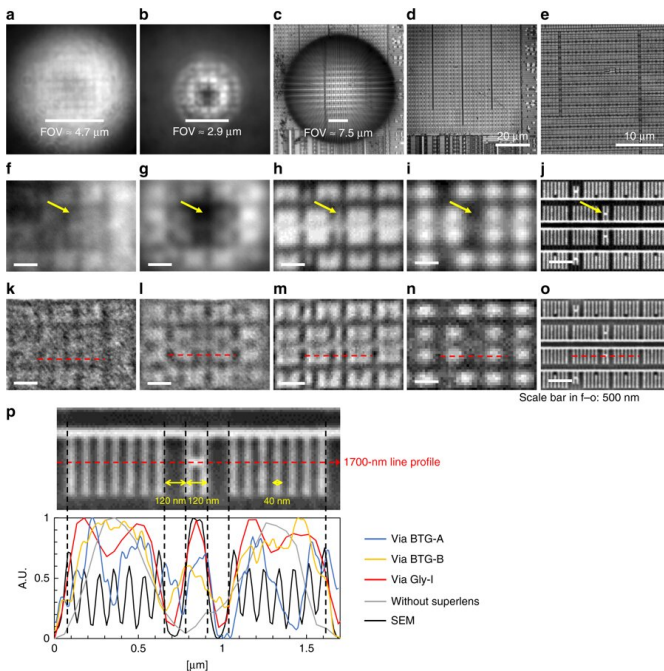
Experimentally acquired images at location-I on the CPU sample. a–d) Optical images taken via BTG-A (a), BTG-B
