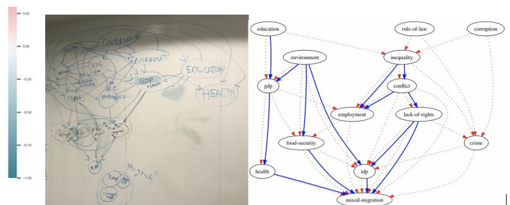
Figure 3: (left) causal network drawn by experts and (right) network learnt based on expert opinion and evidence based on data for all of Sub-Saharan Africa. Credit: IBM
