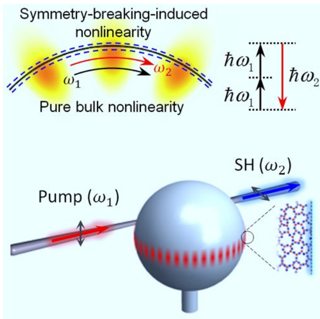
(Upper) Second harmonic is generated from both the symmetry-breaking-induced nonlinearity at the cavity surface and the electric multipole response in the bulk. (Lower) Schematic illustration of the approach to obtain the symmetry-breaking-induced SH signal. Credit: Peking University
