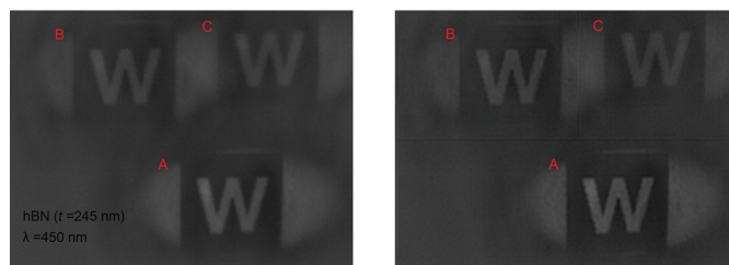
A block letter W imaged by three different prototype metalenses (A, B and C) using different mathematical models — both without (left) and with (right) computational postprocessing. Credit: Liu et al., Nano Letters, 2018
