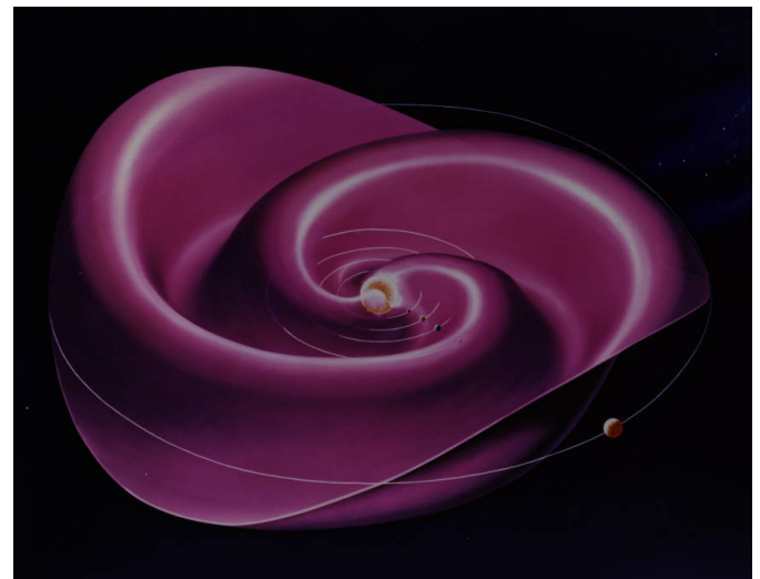
The Sun's magnetic field, which is embedded in the solar wind, permeates the entire solar system. The current sheet -- where the magnetic field changes polarity -- spirals out from near the solar equator like a wavy skirt around a ballet dancer's waist. Credit: NASA's Goddard Space Flight Center
