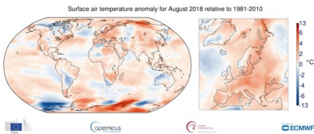
Maps show average temperature for August 2018, relative to 1981-2010 average. Shading indicates warm (red) and cool (blue) areas. Credit: Copernicus Climate Change Service / ECMWF
