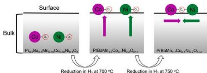
Process of alloy exsolution
