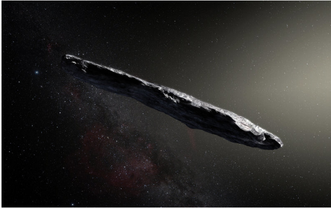
Artist's impression of the interstellar object 'Oumuamua. The object is either elongated as in this image, or else shaped like a pancake. Credit: ESO/M. Kornmesser
