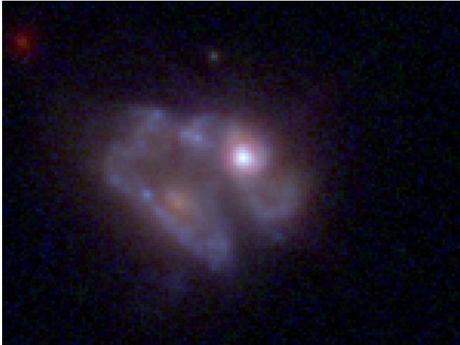
Color Hubble Space Telescope image of 'self-quenching' galaxies 6 billion light years away. The bright dot in the center is the compact area, and some fuzz around the edges tells researchers it's a merger remnant. Credit: KU
