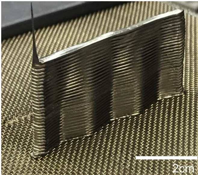
A sample part printed from bulk metallic glass via the TPF-based FFF process. Credit: Elsevier
