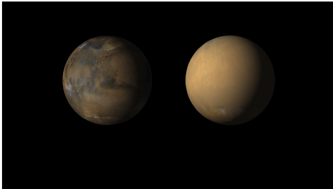
Side-by-side movies shows how dust has enveloped the Red Planet, courtesy of the Mars Color Imager (MARCI) wide-angle camera onboard NASA's Mars Reconnaissance Orbiter (MRO). Credit: NASA/JPL-Caltech/MSSS
