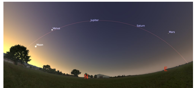
The sky at dusk one evening this week, August 2018. Credit: Stellarium
