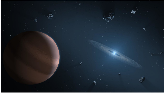
Artists impression of white dwarf star (on right) showing dust disc, and surrounding planetary bodies. Credit: NASA
