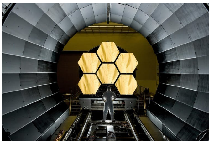
James Webb telescope. Credit: Pixabay
