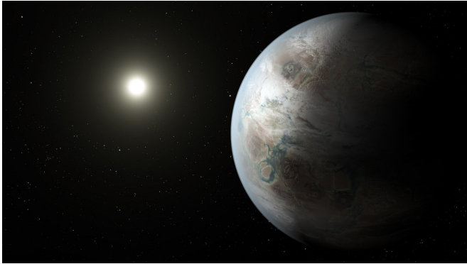
Kepler 452-b is looking like a good candidate for having evolved life. Credit: NASA Ames/JPL-Caltech/T. Pyl
