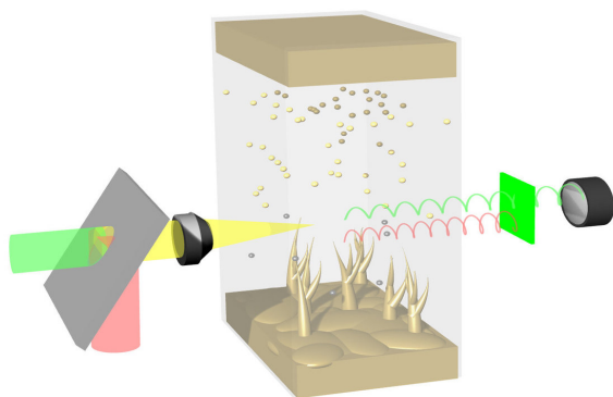
Schematic illustration of a Li-Li symmetric cell under SRS imaging. Credit: Qian Cheng/Columbia Engineering
