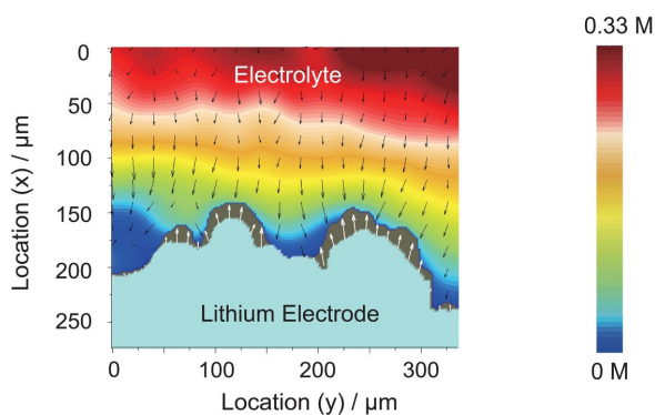
SRS imaging shows the ionic concentration distribution at lithium surface, ionic flux, and lithium deposition at the same time. Credit: Qian Cheng/Columbia Engineering
