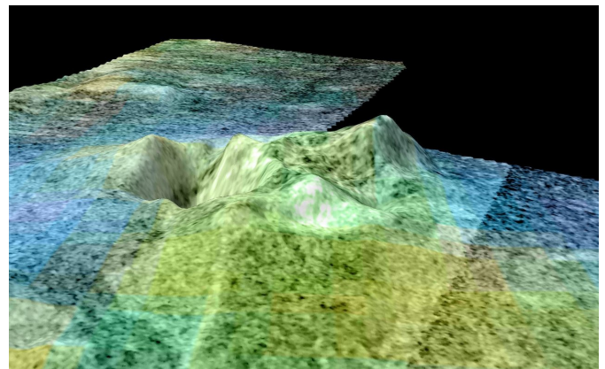
Sotra Facula is a cryovolcano on Titan. This image, built from radar topography with infrared colors overlaid, shows the volcano's caldera, mountainous peaks and thin, bright flows away from the cryovolcano. Credit: NASA/JPL–Caltech/USGS/University of Arizona
