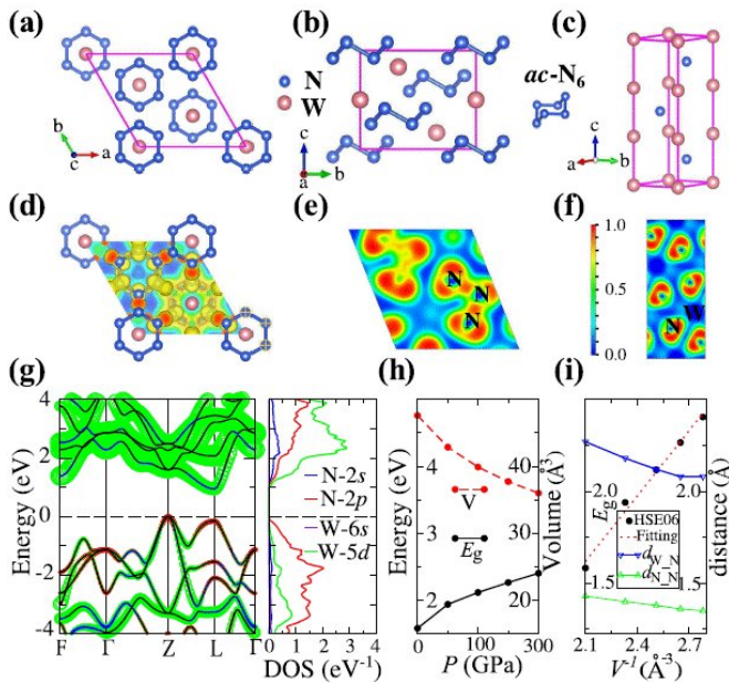
Crystal structure and theoretical electronic structures of new W-N phases. Credit: ©Science China Press
