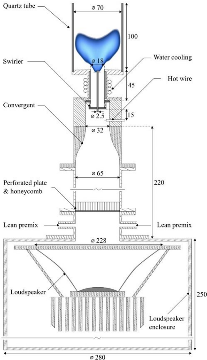
A loudspeaker generates the sound waves that test how acoustic perturbation affects the gas flame. Credit: Reproduced with permission from reference 1. Figure 1a. © 2018 Elsevier
