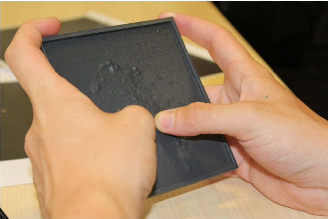
A 3D printed model of a galaxy. Credit: University of Portsmouth
