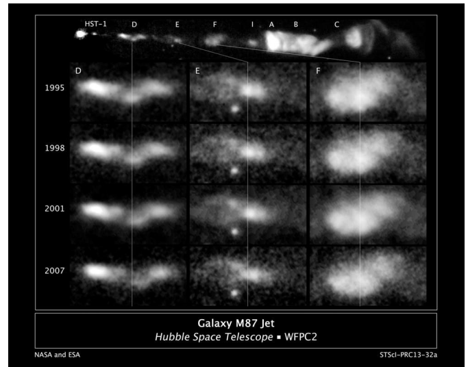
A black-hole-powered jet of hot gas in the giant elliptical galaxy M87. Credit: NASA, ESA, E. Meyer, W. Sparks, J. Biretta, J. Anderson, S.T. Sohn, and R. van der Marel (STScI), C. Norman (Johns Hopkins University), and M. Nakamura (Academia Sinica)
