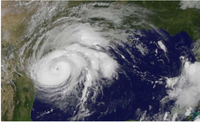
An image of Hurricane Harvey taken by the GOES-16 satellite as the storm collided with the Texas coast. Credit: NASA.
