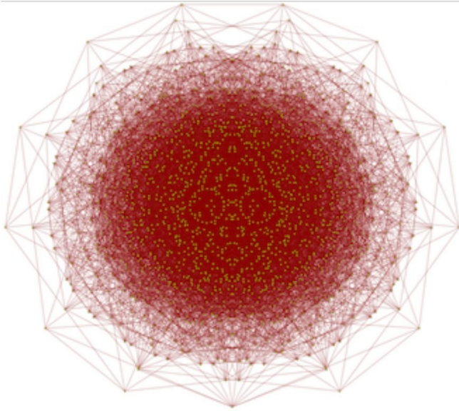
The 1581-vertex, non-4-colourable unit-distance graph G. Credit: arXiv:1804.02385 [math.CO]
