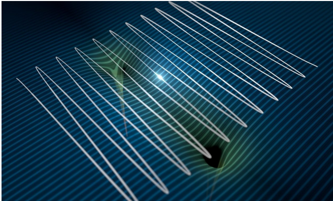
Schematic illustration of the Kramers Henneberger potential formed by a mixture of the atomic potential and a strong laser field. Credit: UNIGE - Xavier Ravinet
