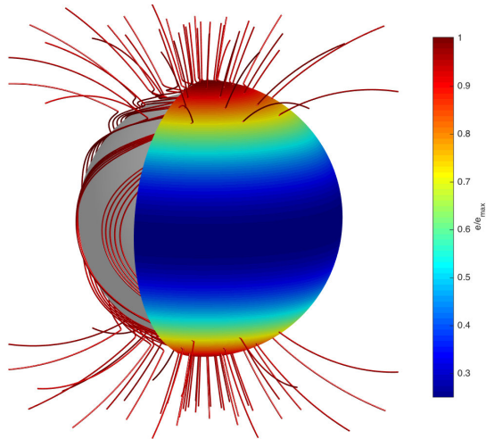
A tightly wound-up magnetic field used as initial state in the simulation. Credit: K. Gourgouliatos, R. Hollerbach, U. Durham, U. Leeds
