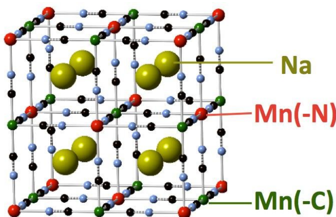
Atomic structure of the anode material that achieved high performance in a sodium-ion battery. Sodium (Na) atoms and manganese (Mn) atoms are labeled. Credit: Berkeley Lab
