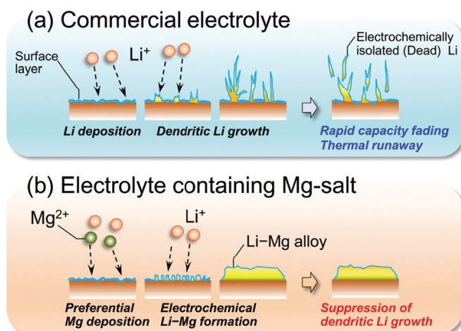
Schematic illustration of the proposed suppressing effect of Li dendritic growth by addition of Mg-salt. Credit: Royal Society of Chemistry
