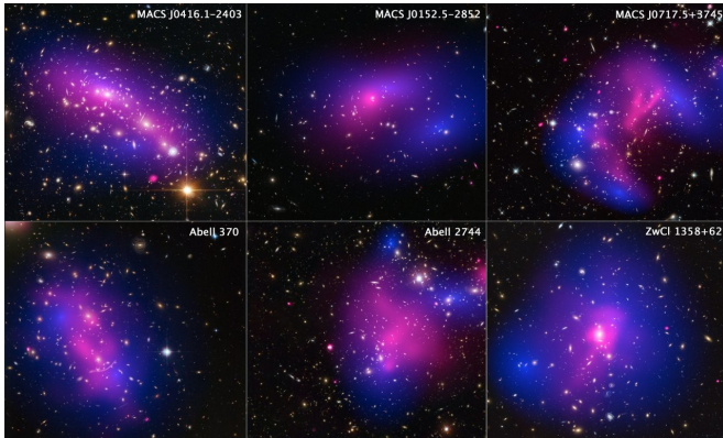
The distribution of dark matter (colored in blue) in six galaxy clusters, mapped from the visible-light images from the Hubble Space Telescope. (Source: NASA, ESA, STScI, and CXC) Credit: NASA, ESA, STScI, and CXC
