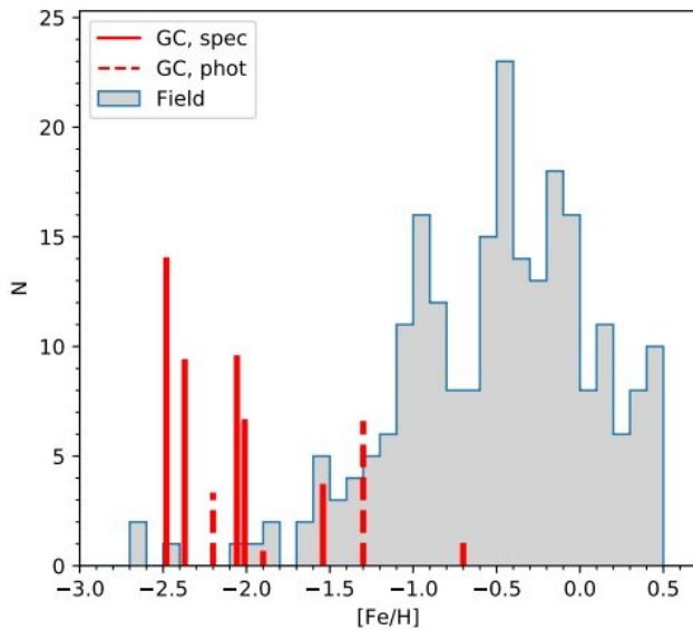
Metallicity distributions of field stars (Ho et al. 2014) and GCs in NGC 147. For the GCs, the bars have been scaled according to the V-band luminosity of each cluster. Solid bars: this work. Dashed bars: Veljanoski et al. (2013). Credit: Larsen et al., 2018.
