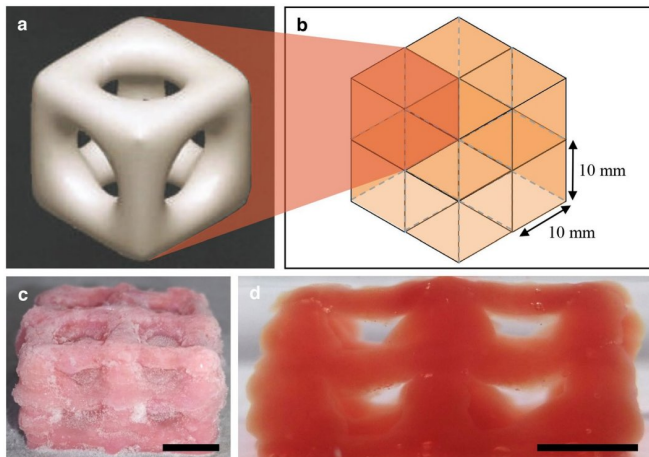
Structure of a single unit; how eight units fit together; two views of a printed and set eight-unit structure. Credit: Imperial College London
